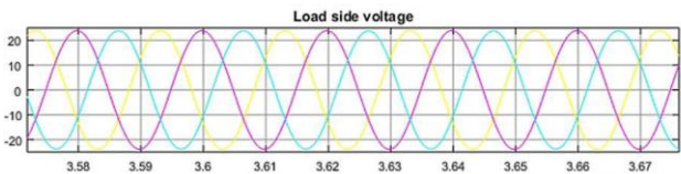
Fig.5.4. Load side voltage (HSAPF)
