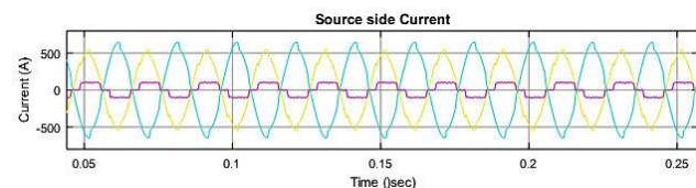
Fig.5.5. Source side current (SAPF)
