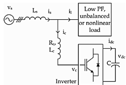
Fig.1.1 voltage source active power filter
