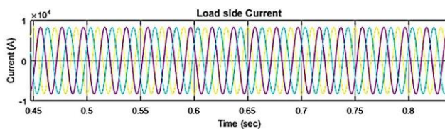
Fig.5.8. Load side current (HSAPF)
