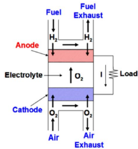
Figure 1.1: Basic configuration of Fuel Cell with operation
