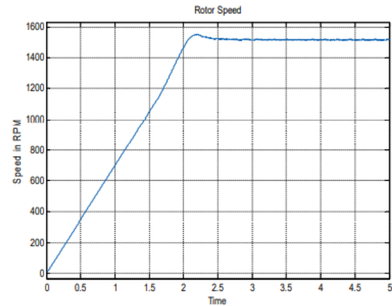
Figure 5.2: Rotor Speed of the Single phase Split Phase Induction Motor with proposed System
