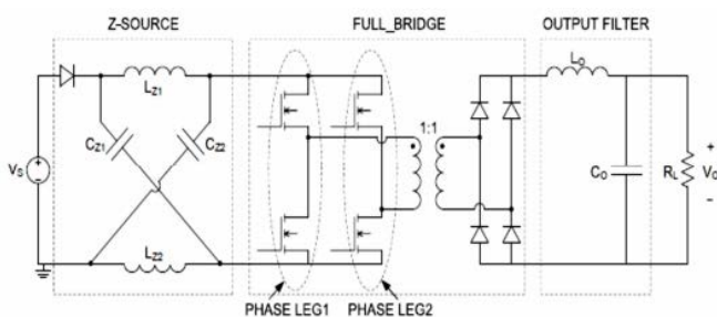
Figure 4.1: Circuit diagram of the Z-source full bridge dc/dc converter
