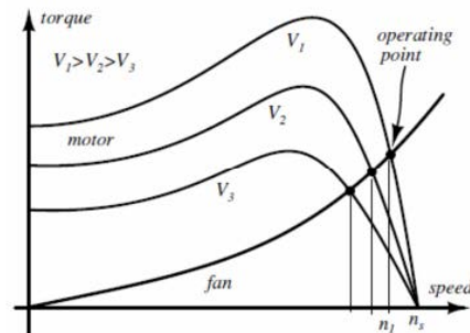
Figure 1.4: Torque-speed characteristics of an induction motor and fan load with variable voltage.
