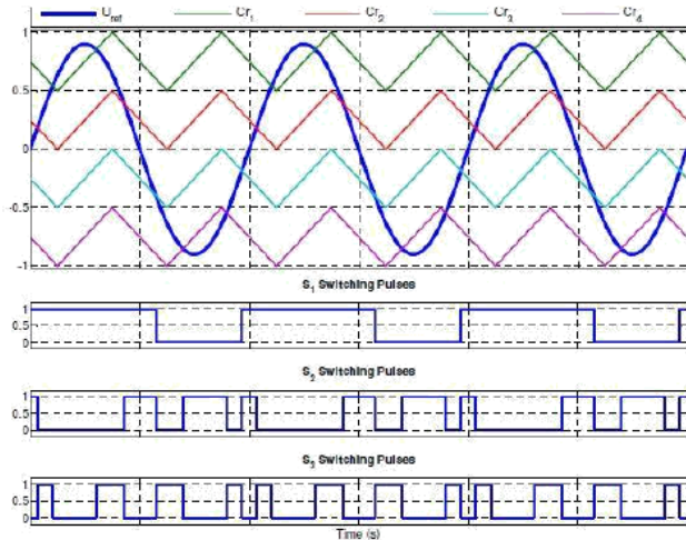
Figure 5.2 Proposed multicarrier PWM technique for low and fixed switching frequency purposes
