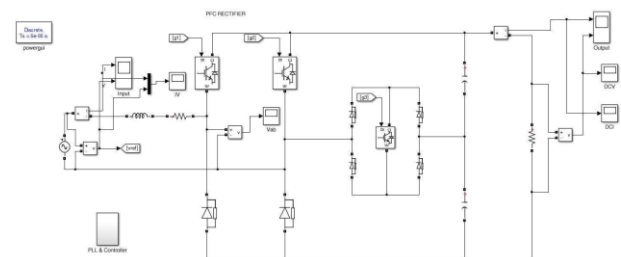
Figure 5.1 Model of the proposed system
