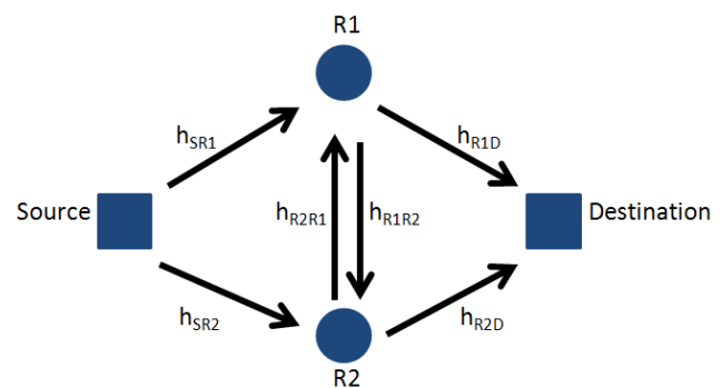
Figure 1.1 A simple Cooperative relay network.
