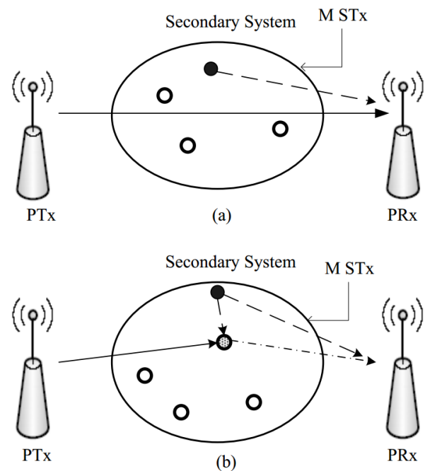
Figure 3.1 Cooperative Hybrid Sharing System.
