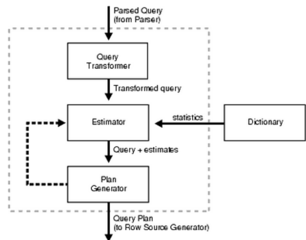
Figure 1.1: Steps in query processing
