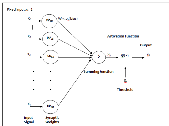
Fig 3. Mathematical model of artificial neural network
