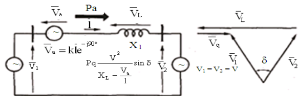
Fig.1. Basic model of the series compensation with a voltage source
