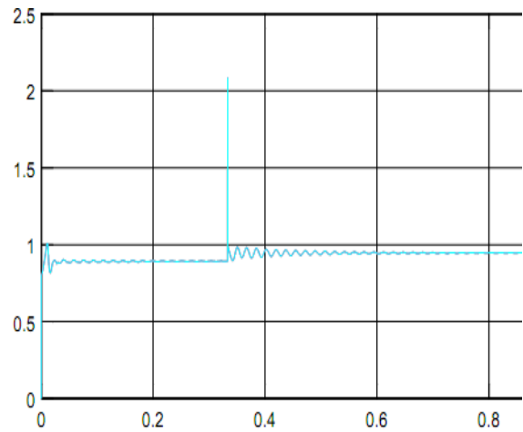
Fig.10. SSSC D.C voltage with fuzzy logic control
