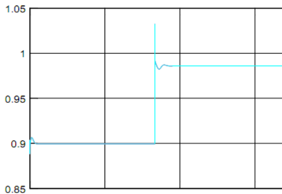
Fig.7. Line voltage with PI control
