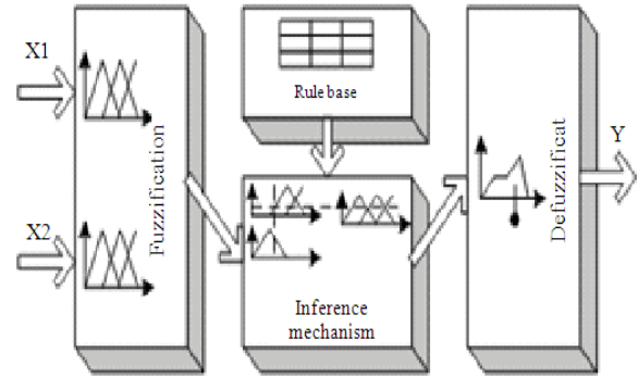
Fig.3. The structure of the fuzzy logic controller
