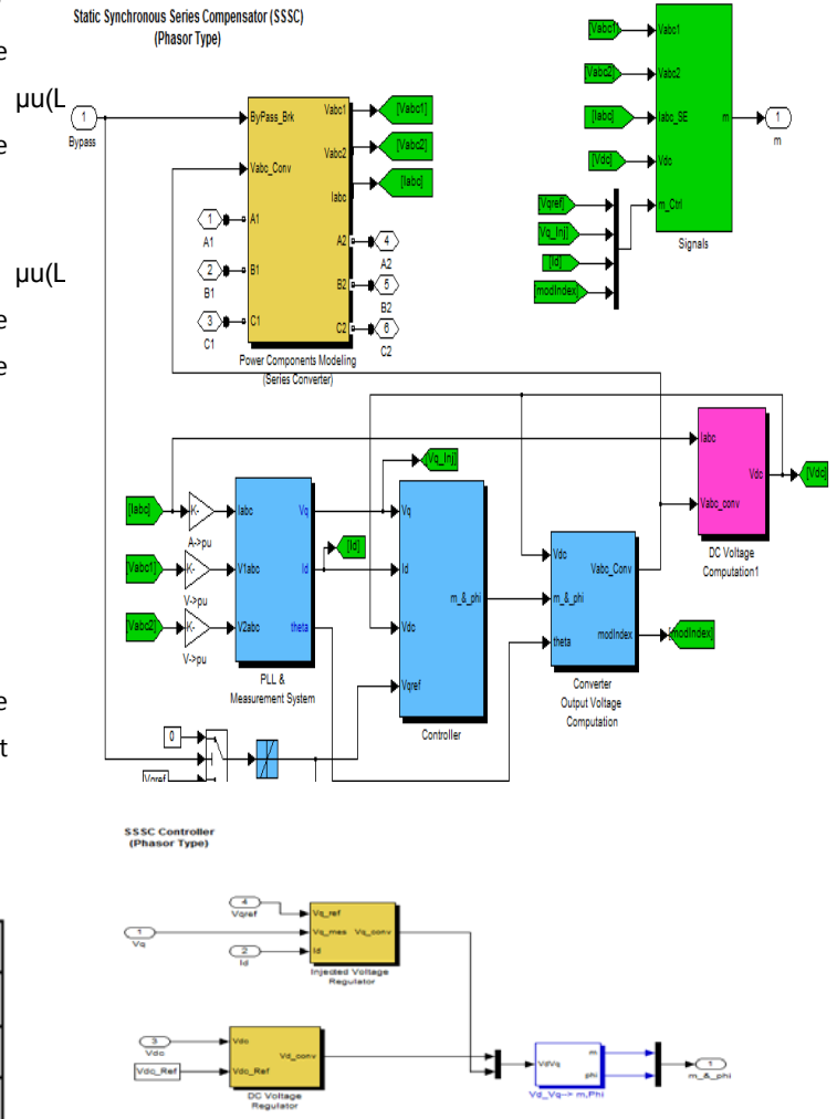
Fig.4. SSSC phasor control model
