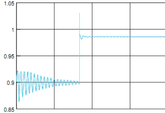
Fig.8. Line voltage with fuzzy logic control
