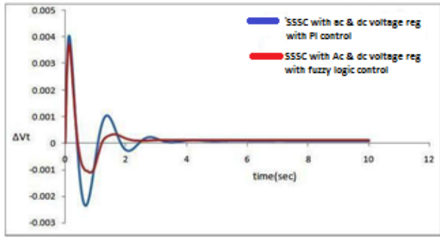
Fig.11. Voltage regulation comparison and transient analysis
