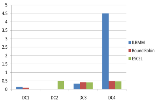
Figure6. Data Center Request Servicing Timing
