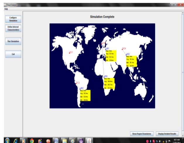
Figure 4. Cloud Analyst Main Result Screen
