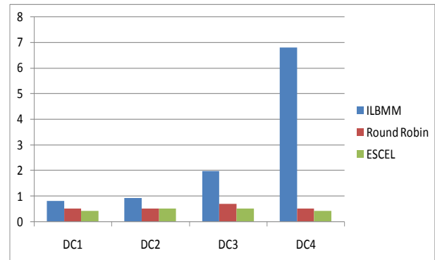
Figure7. Cost of VM
