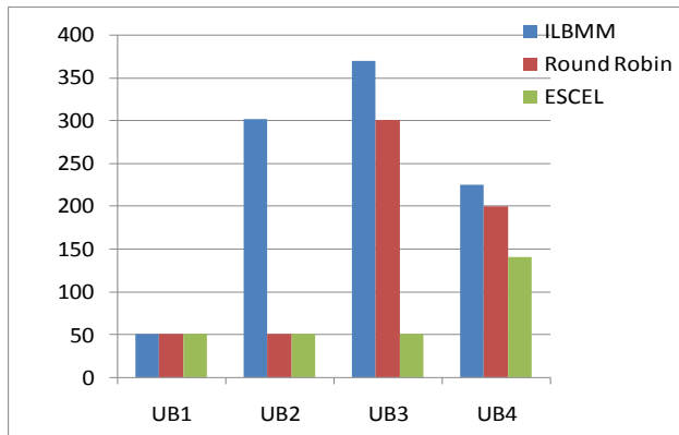
Figure 5. Response Time observed by user
