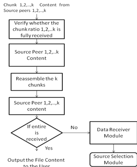
Fig.13. Data Receiver Module
