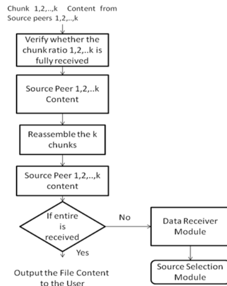
Fig.8. Data Receiver Module
