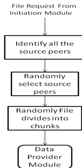
Fig.5. Source Selection Function Module
